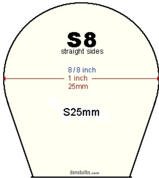
typical shape of S8 glass envelopes (not to scale)
