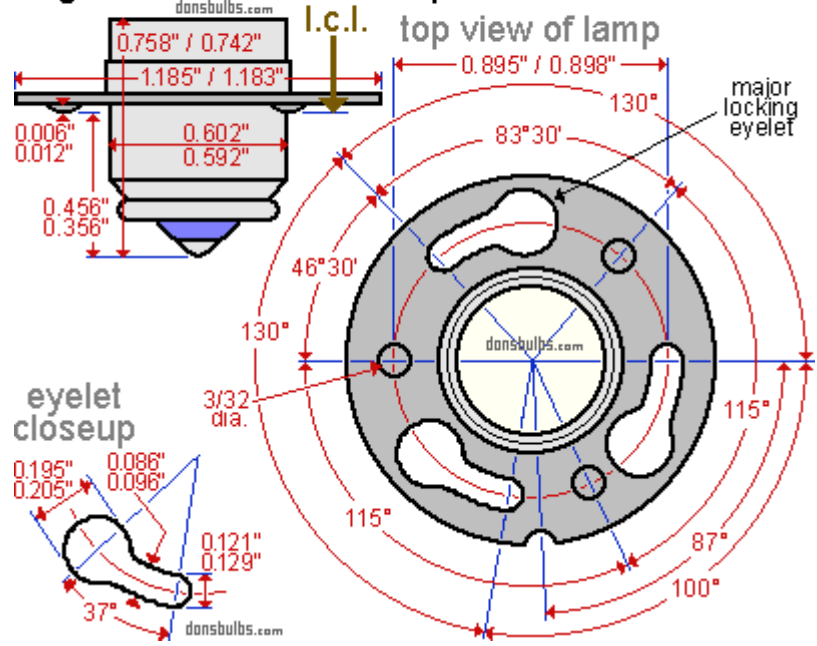
industry standards for base: P15s30 - Single Contact Prefocus Flanged also known as Single Contact Prefocus Bayonet also known as P15s (Europe) also known as P30s (USA) (not to scale)
