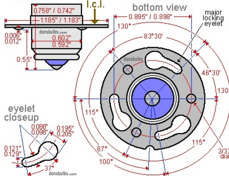
Industry standards for base: P15s30B (not to scale)
