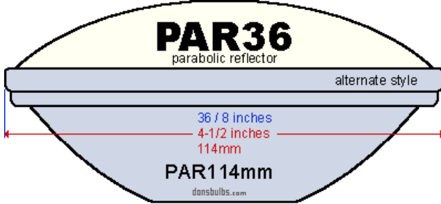
typical photo of 4416 12.8V 30W USA bulb type (your bulb may look slightly different)
