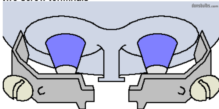
industry standards for base: ST2 (not to scale)
