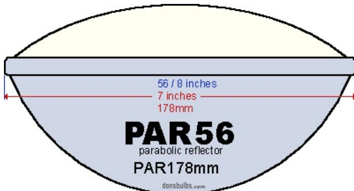
typical shape of PAR56 glass envelopes (not to scale)
