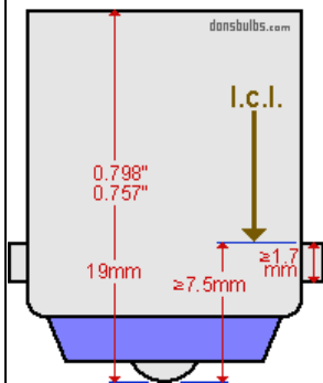
industry standards for base: BA15s - Single Contact Candelabra Bayonet (or S.C.Bayonet) (not to scale)
