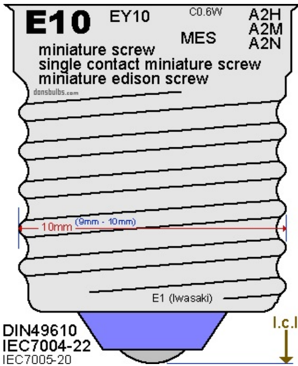
industry standards for base: E10 - Edison Miniature Screw, 10mm (not to scale)
