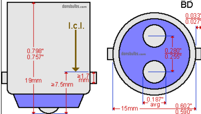
industry standards for base: BA15d - Double Contact Candelabra Bayonet (or D.C.Bayonet) (not to scale)
