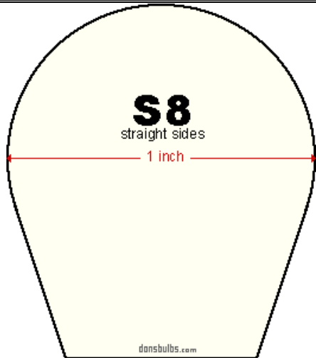
usual shape of S8 glass envelopes (not to scale)
