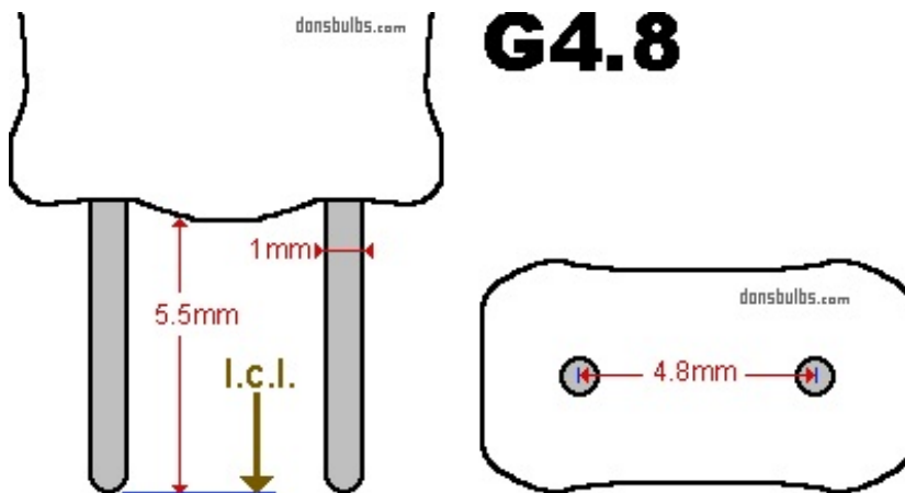
industry standards for base: G4.8 (not to scale)
