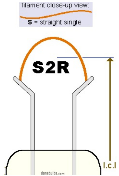
typical shape of S2R filament
