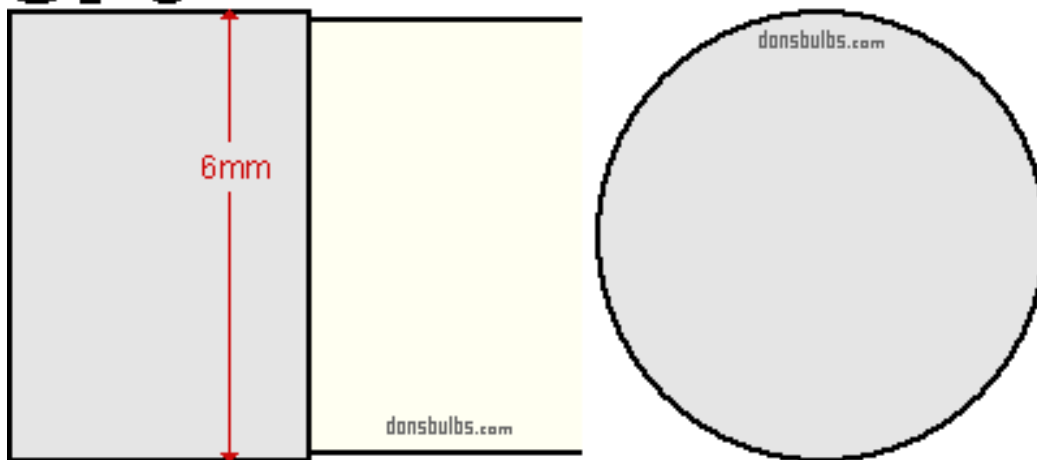
industry standards for base: SF6 (not to scale)
